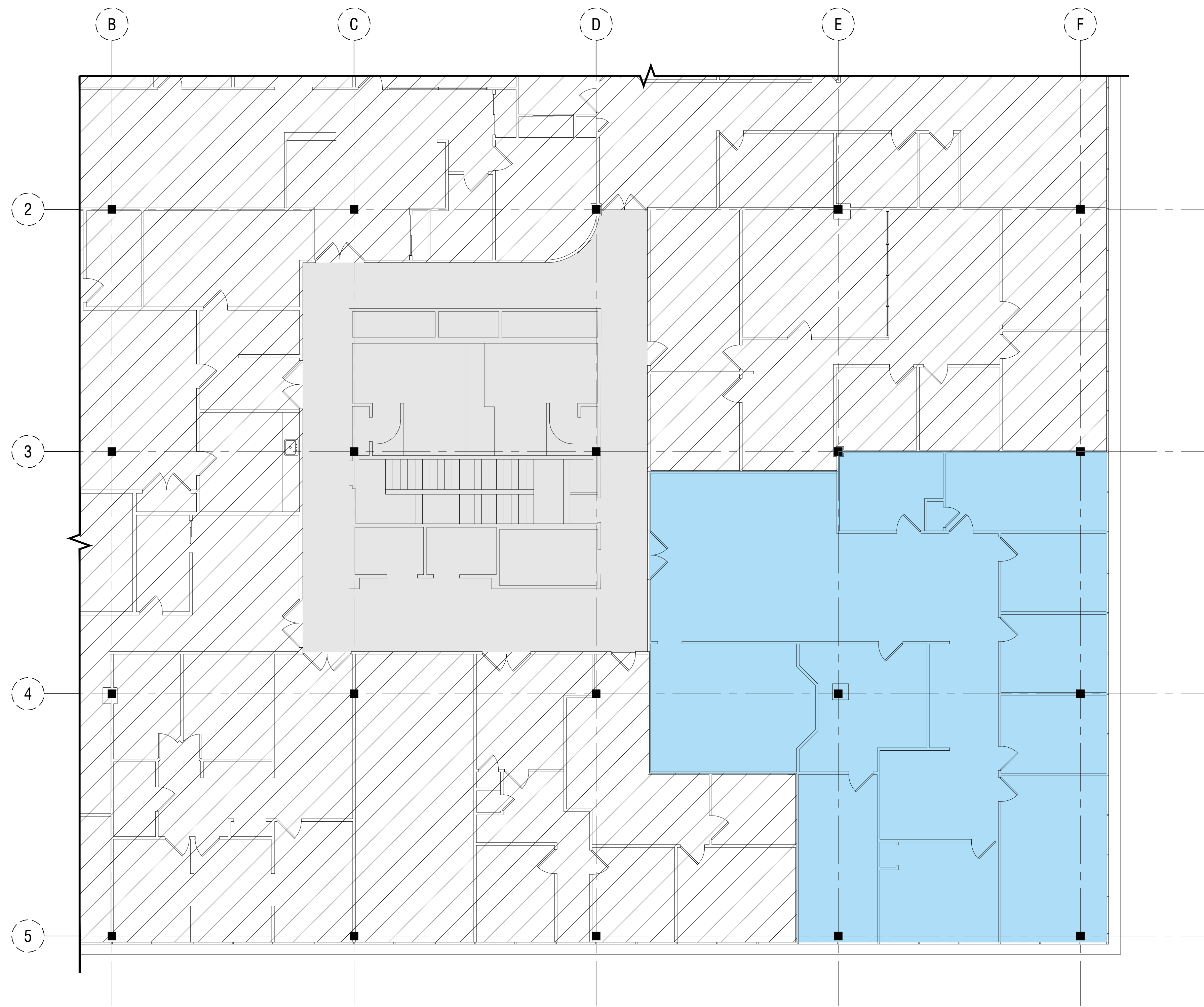
1 FLOOR PLAN - 5TH FLOOR 1/8" = 1'-0"
